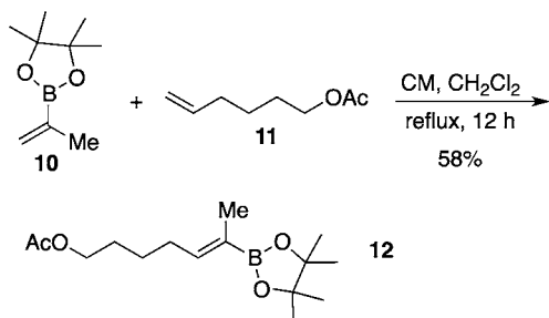
Scheme 4. Successful Cross-Metatheses of 3
