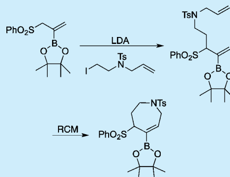
Scheme 1. RCM of a Boronate
