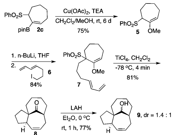
Scheme 2. From Cyclic Boronate to (4 + 3)-Cycloadduct
