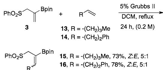
Scheme 4. Successful Cross-Metatheses of 3
